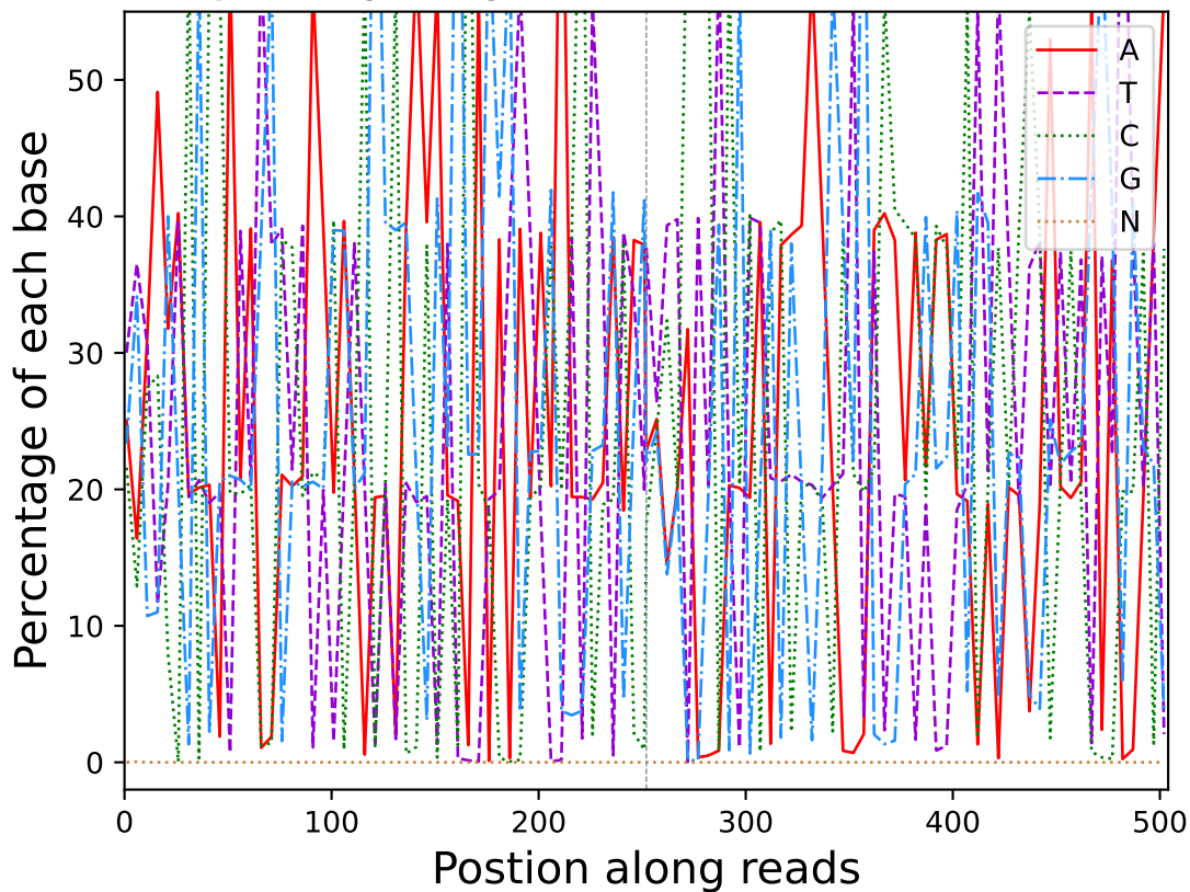
Base percentage along reads (R20103)
